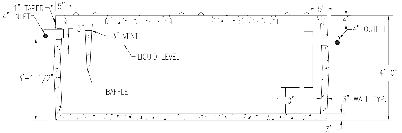
SECTION
